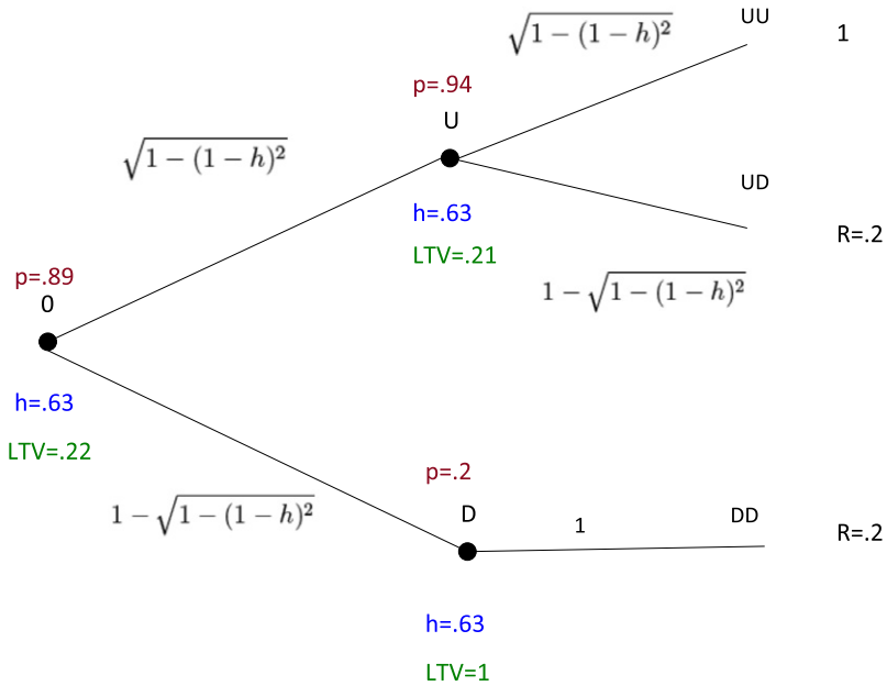
Fig. 9. Extreme GV equilibrium for R = .2 .
